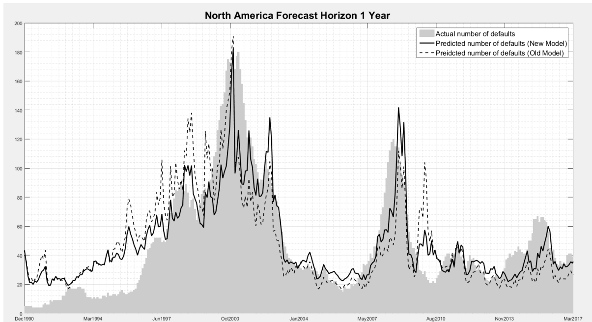
Figure 1: Actual number of defaults in North America and predicted number of defaults
