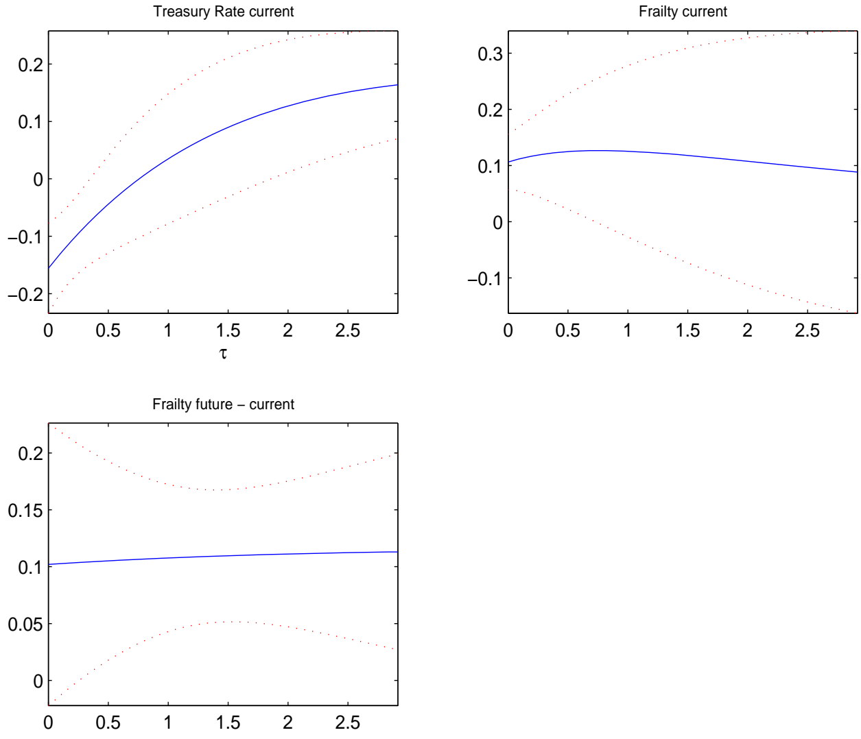
This figure shows the parameter estimates for the forward default intensity function corresponding to different prediction horizons under the PC-F model. “Treasury Rate” is the 3-month US Treasury rate, “Frailty” is the common latent factor. The solid blue curve is for the parameter estimates and the dotted red curves depict the 90% confidence interval.
