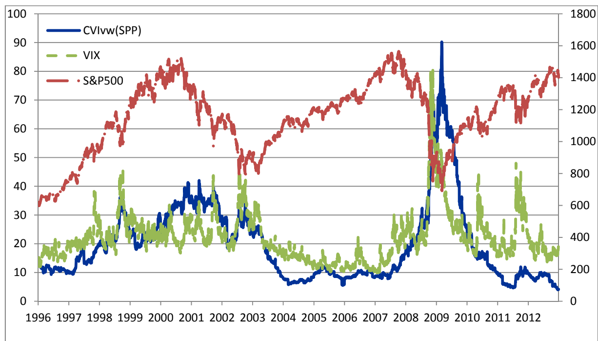
Figure 1: A comparison of the CVI_{vw} (SPP), VIX and S&P 500 index.
