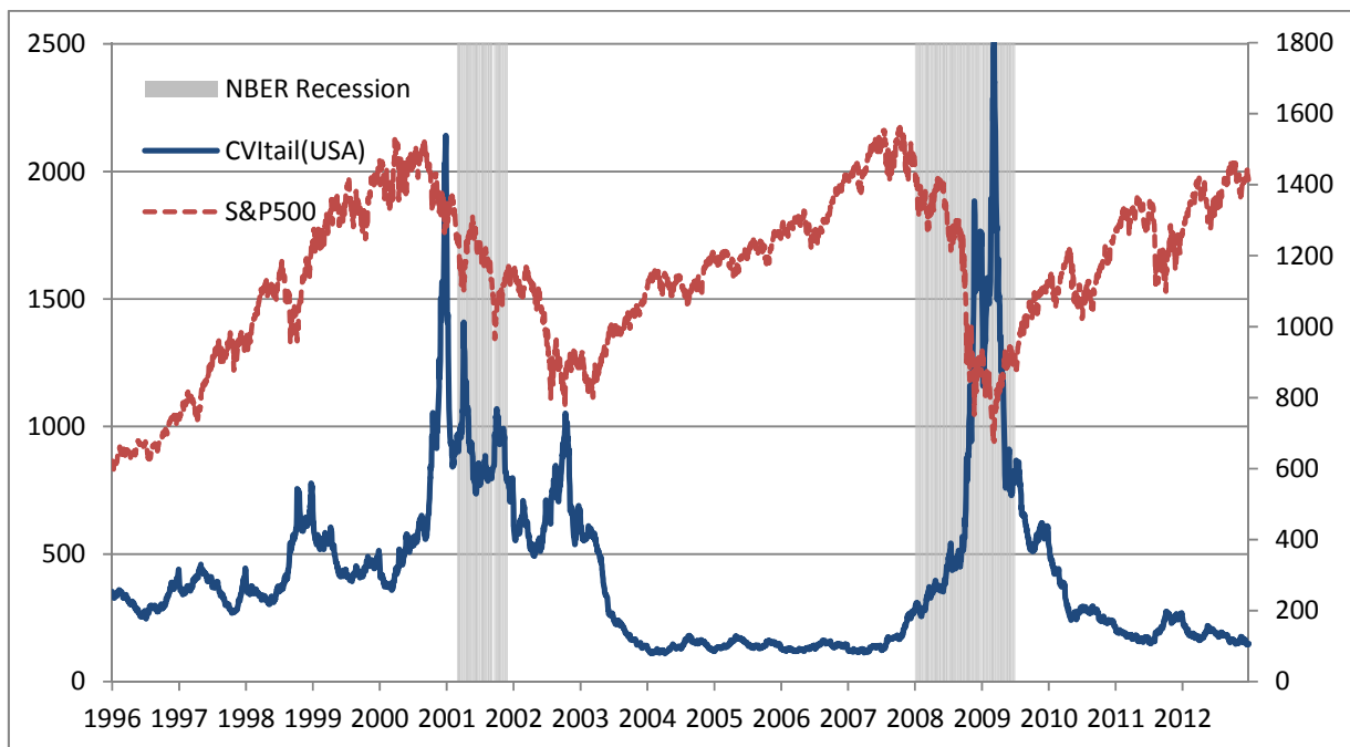
Figure 4: A comparison of CVI_{tail}(USA) and S&P 500 index during NBER recessions.
