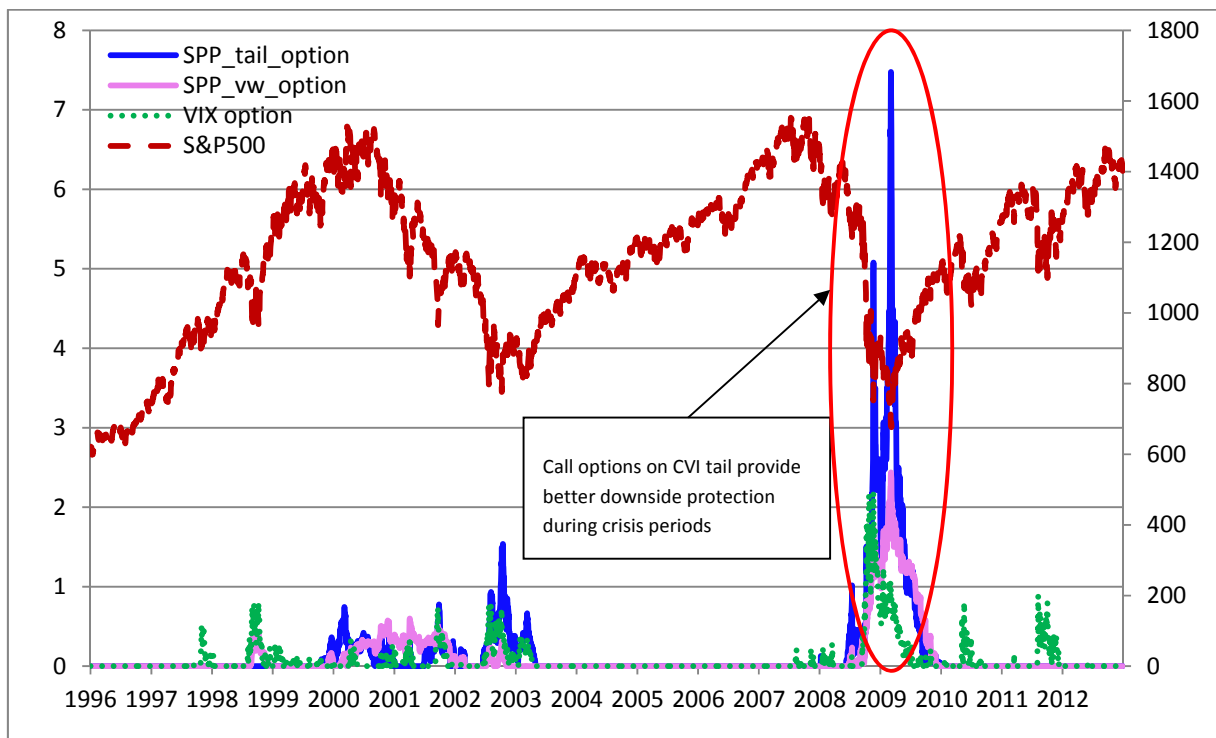
Figure 5: A comparison of the daily scaled payoffs of synthetic one-year CVI_{tail}(SPP) call option, one-year VIX call option and the S&P 500 index.
